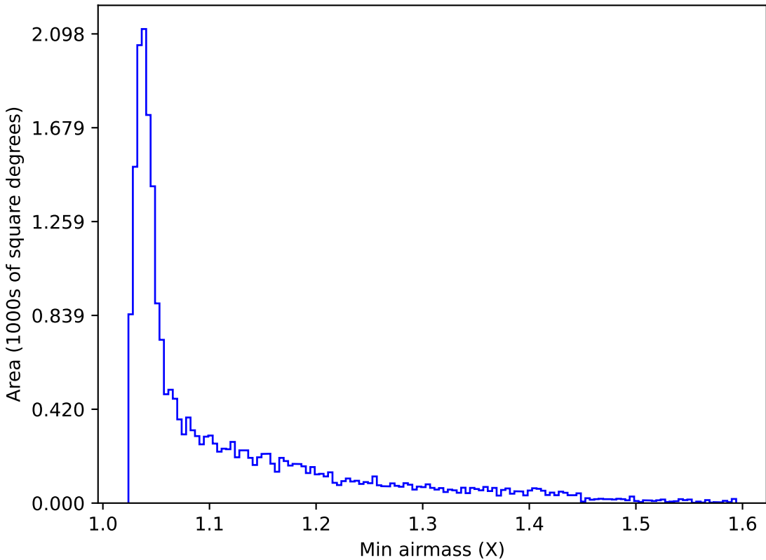
ddf_loaded_fl2_v3.4_10yrs All sky u band: Min airmass
