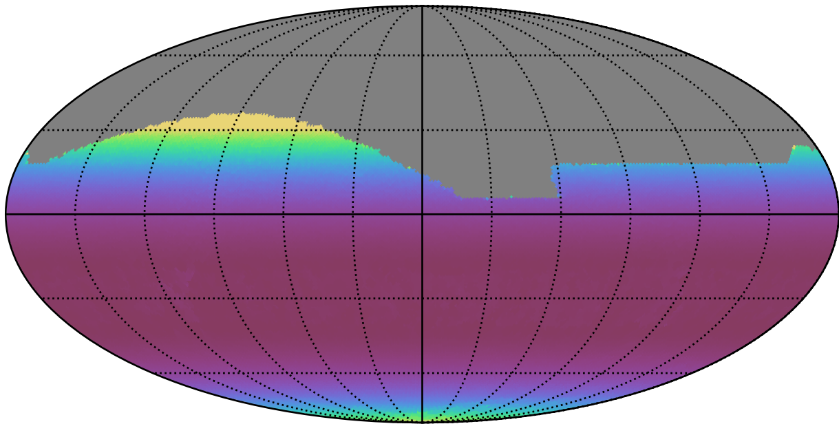
ddf_loaded_fl2_v3.4_10yrs All sky r band: Min airmass
