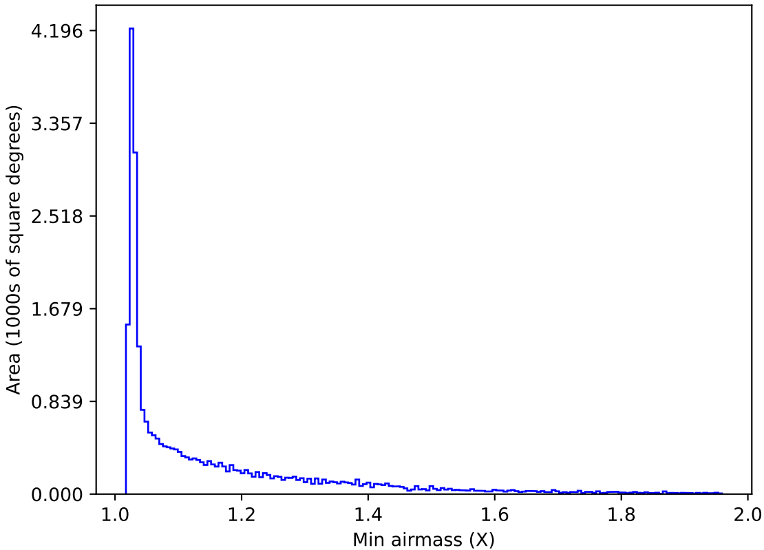
ddf_loaded_fl2_v3.4_10yrs All sky r band: Min airmass
