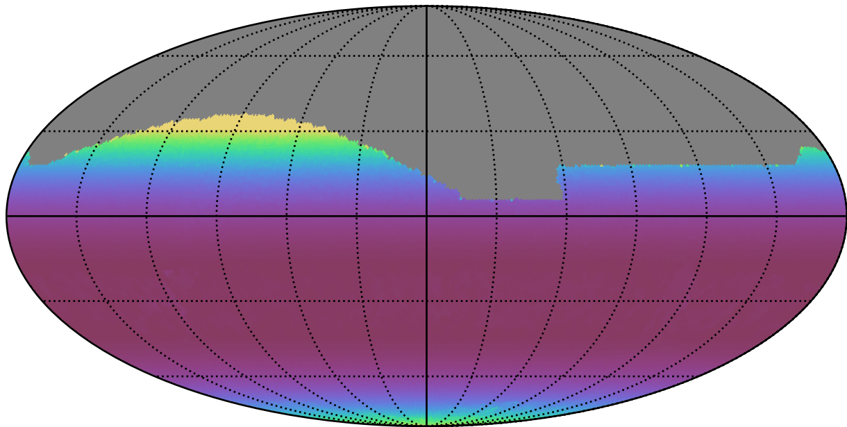
ddf_loaded_fl2_v3.4_10yrs All sky i band: Min airmass
