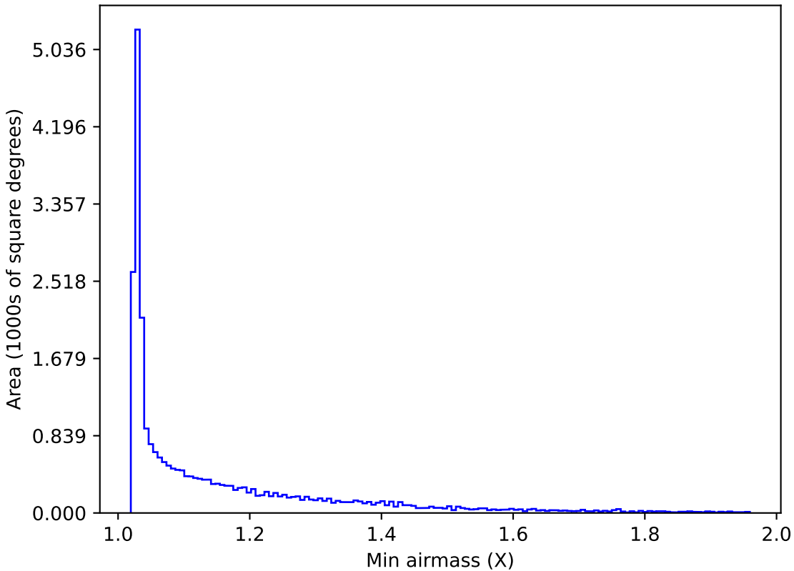
ddf_loaded_fl2_v3.4_10yrs All sky i band: Min airmass
