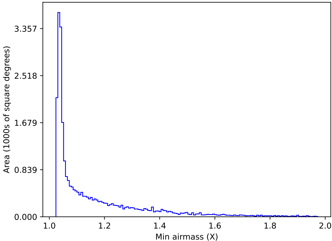
ddf_loaded_fl2_v3.4_10yrs All sky g band: Min airmass
