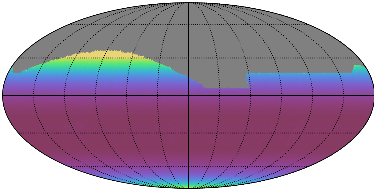
ddf_loaded_fl2_v3.4_10yrs All sky all bands: Min airmass
