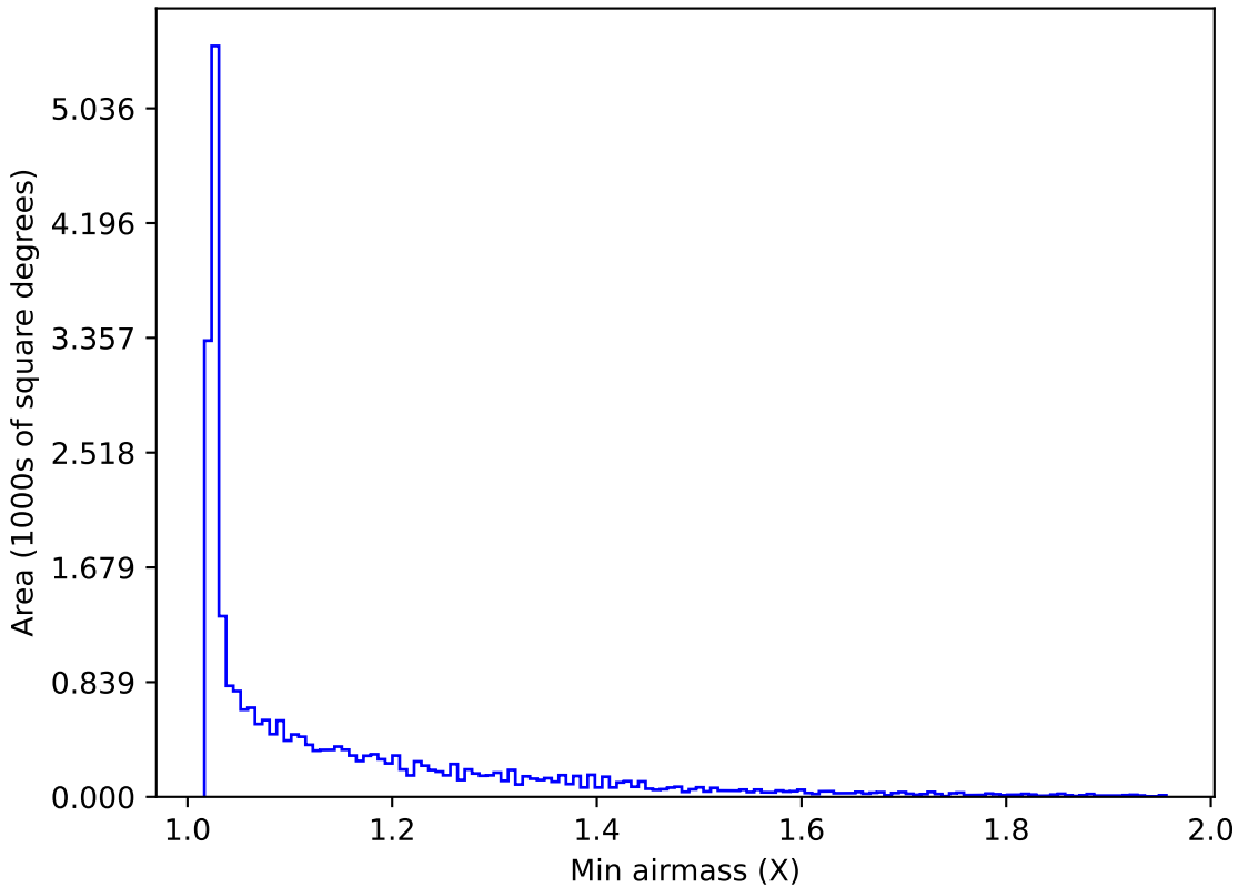
ddf_loaded_fl2_v3.4_10yrs All sky all bands: Min airmass
