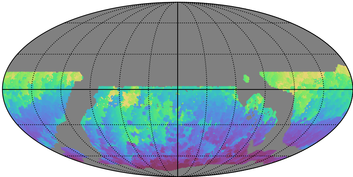
ddf_loaded_fl2_v3.4_10yrs WFD z band: Min HA
