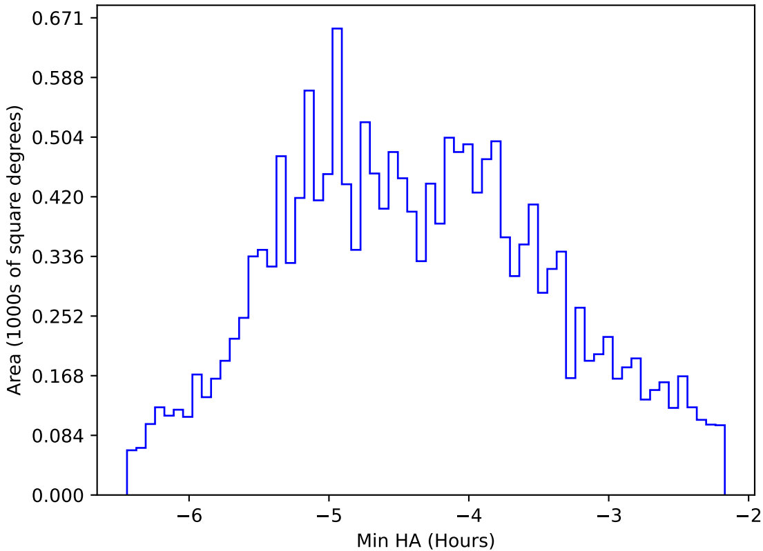
ddf_loaded_fl2_v3.4_10yrs WFD z band: Min HA
