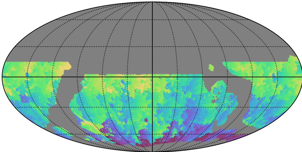
ddf_loaded_fl2_v3.4_10yrs WFD u band: Min HA
