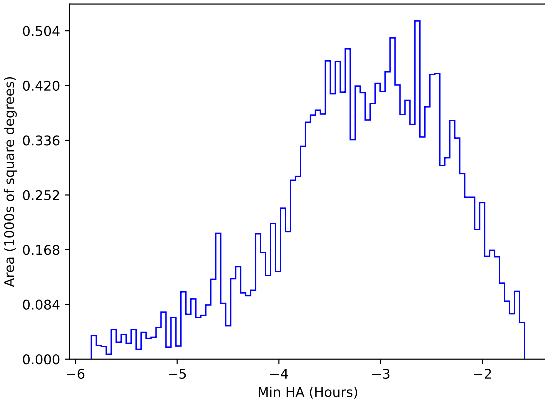
ddf_loaded_fl2_v3.4_10yrs WFD u band: Min HA
