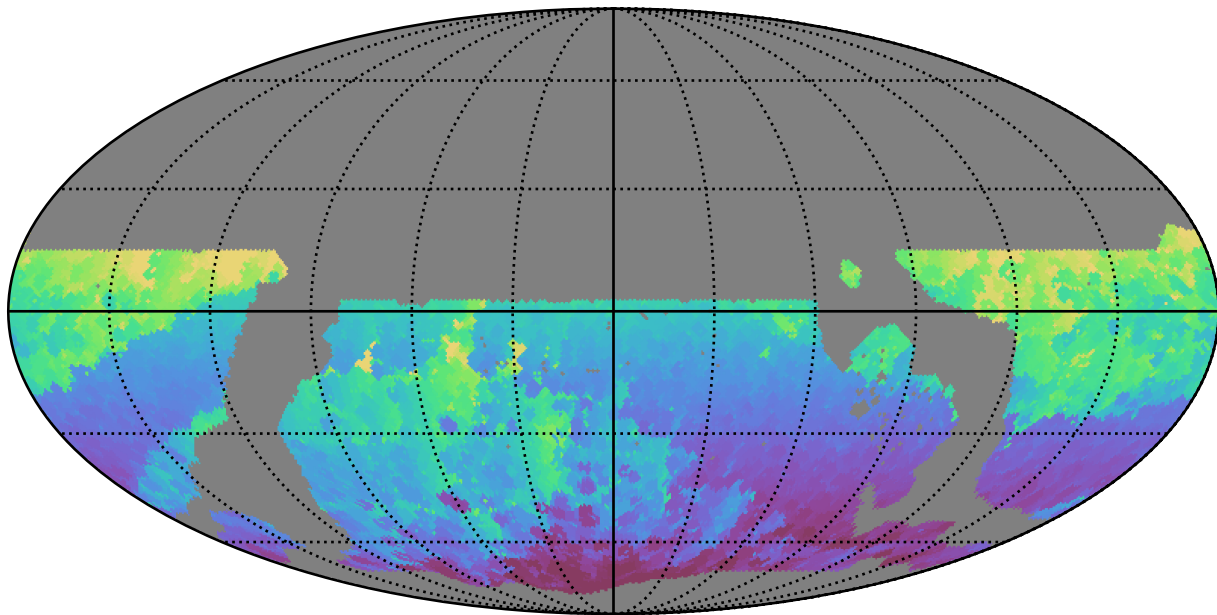
ddf_loaded_fl2_v3.4_10yrs WFD r band: Min HA
