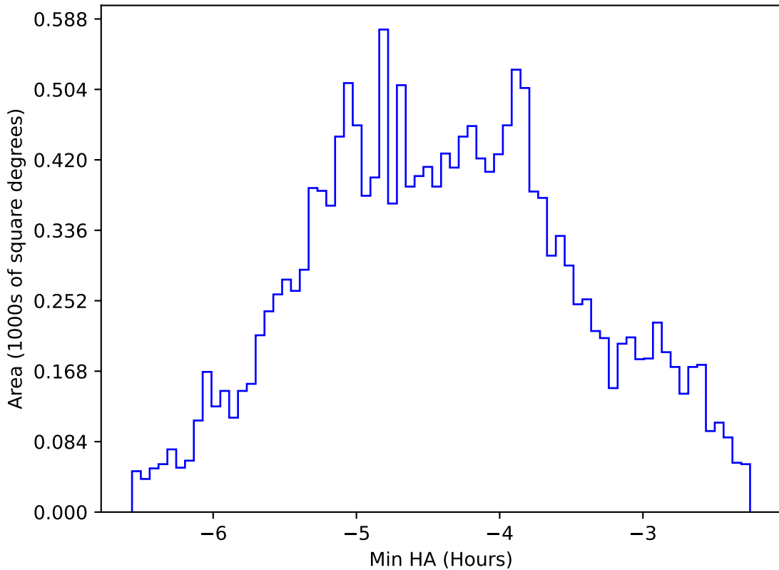
ddf_loaded_fl2_v3.4_10yrs WFD i band: Min HA
