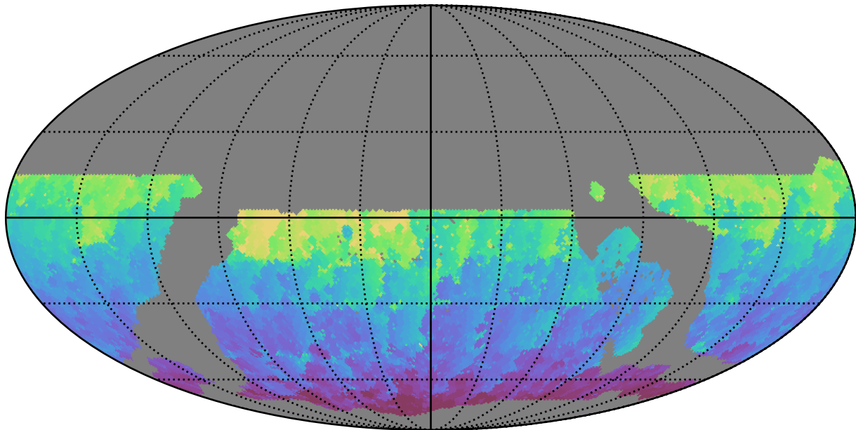
ddf_loaded_fl2_v3.4_10yrs WFD g band: Min HA
