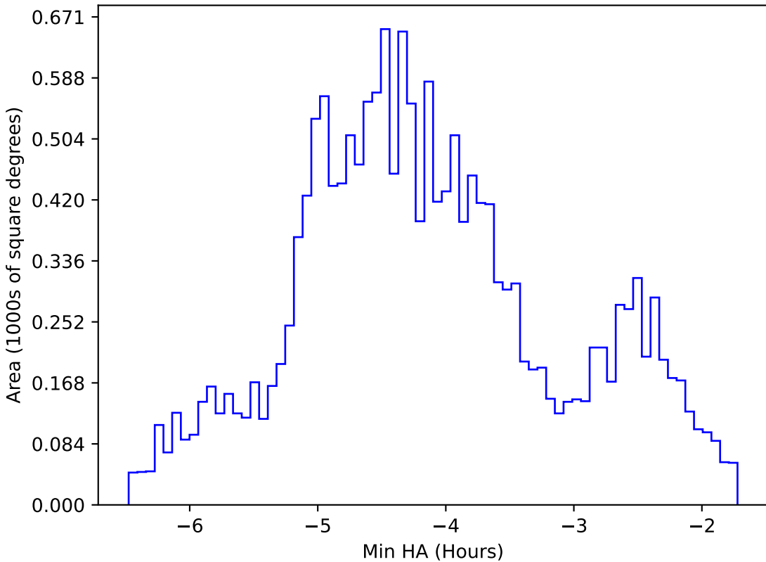
ddf_loaded_fl2_v3.4_10yrs WFD g band: Min HA
