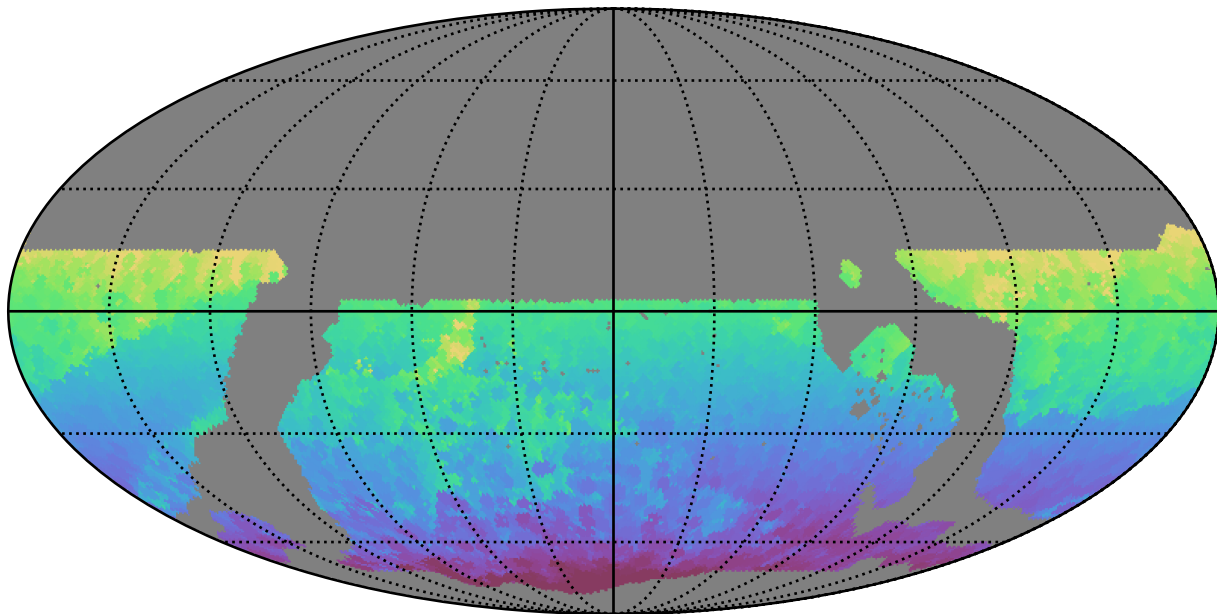
ddf_loaded_fl2_v3.4_10yrs WFD all bands: Min HA
