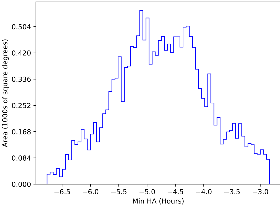
ddf_loaded_fl2_v3.4_10yrs WFD all bands: Min HA
