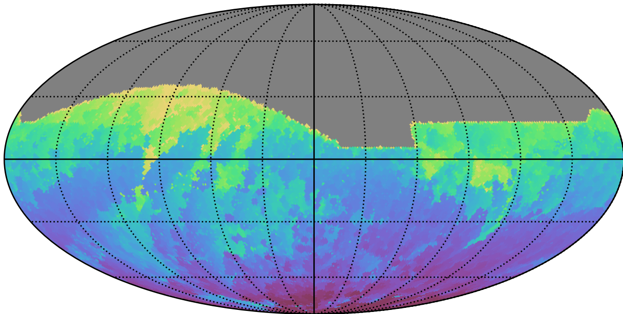
ddf_loaded_fl2_v3.4_10yrs All sky z band: Min HA
