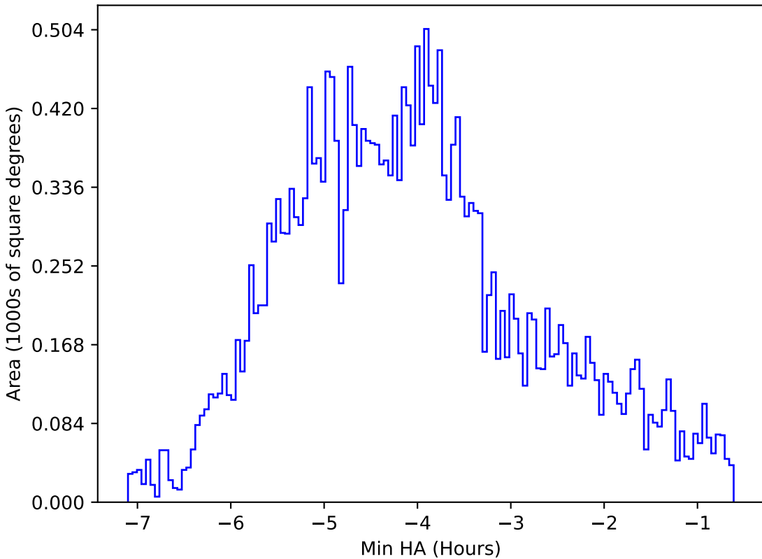
ddf_loaded_fl2_v3.4_10yrs All sky z band: Min HA
