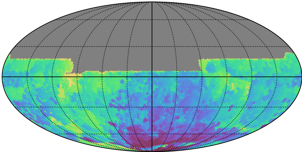
ddf_loaded_fl2_v3.4_10yrs All sky y band: Min HA
