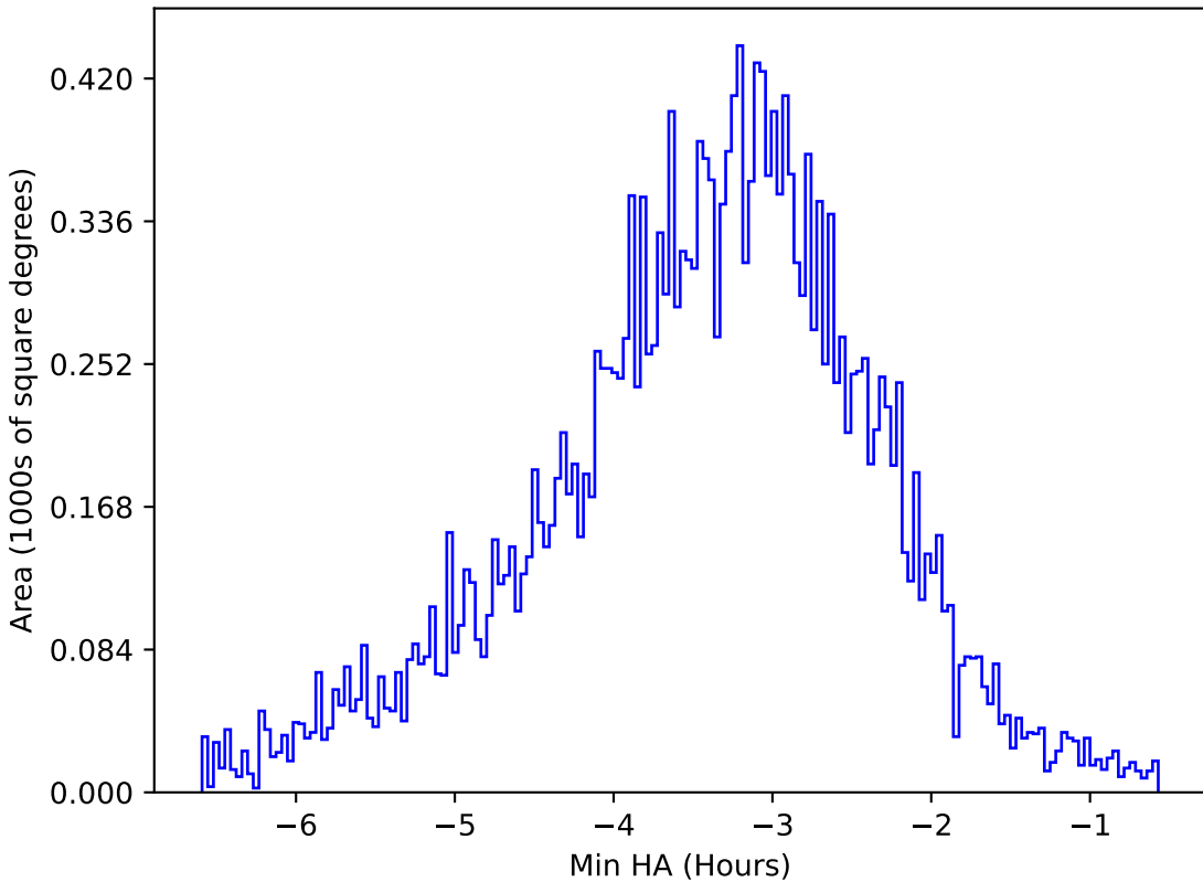
ddf_loaded_fl2_v3.4_10yrs All sky y band: Min HA
