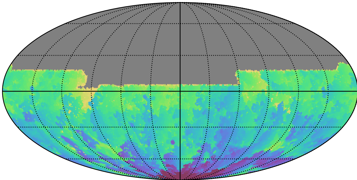
ddf_loaded_fl2_v3.4_10yrs All sky u band: Min HA
