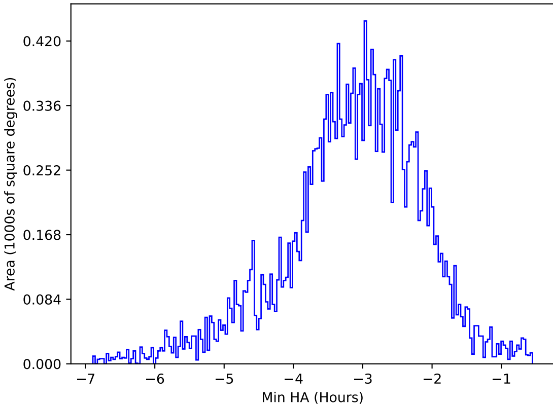
ddf_loaded_fl2_v3.4_10yrs All sky u band: Min HA
