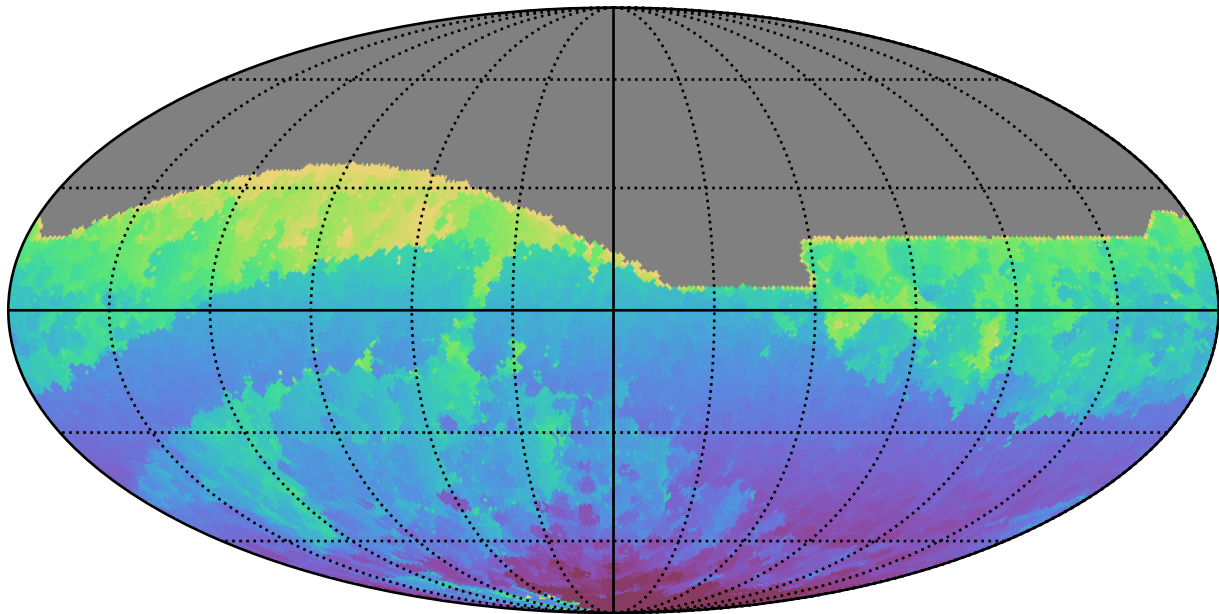
ddf_loaded_fl2_v3.4_10yrs All sky r band: Min HA
