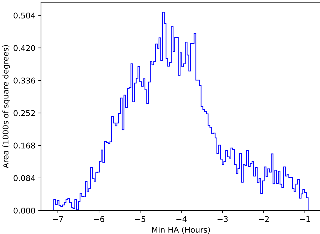
ddf_loaded_fl2_v3.4_10yrs All sky r band: Min HA
