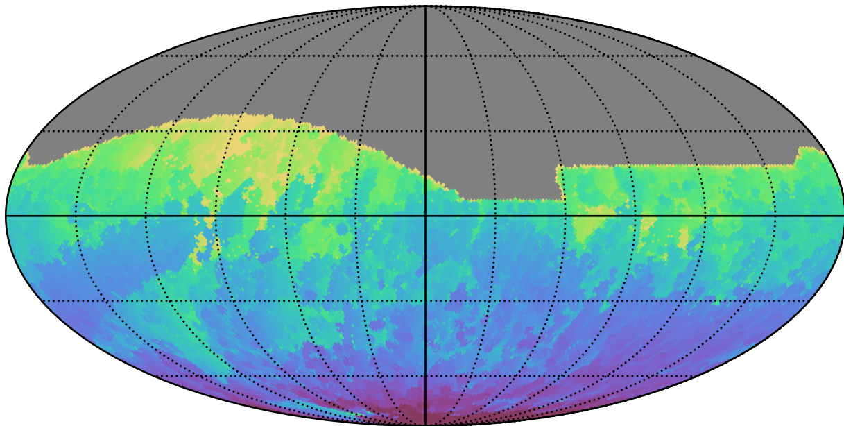
ddf_loaded_fl2_v3.4_10yrs All sky i band: Min HA
