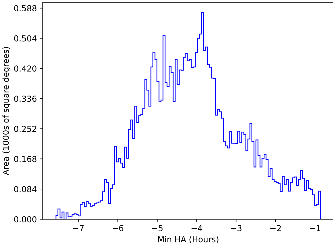
ddf_loaded_fl2_v3.4_10yrs All sky i band: Min HA
