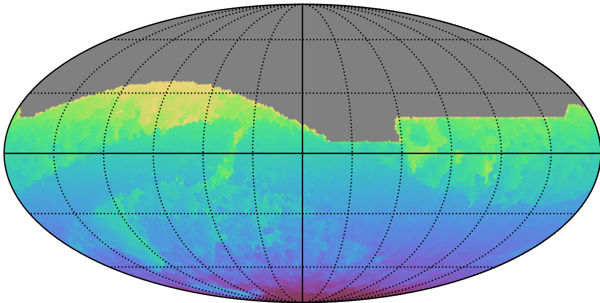
ddf_loaded_fl2_v3.4_10yrs All sky all bands: Min HA
