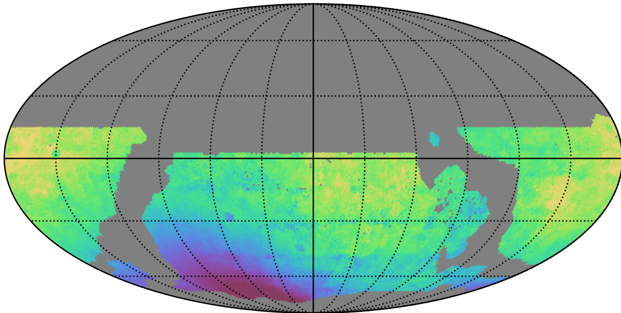
ddf_loaded_fl2_v3.4_10yrs WFD z band: Median solarElong
