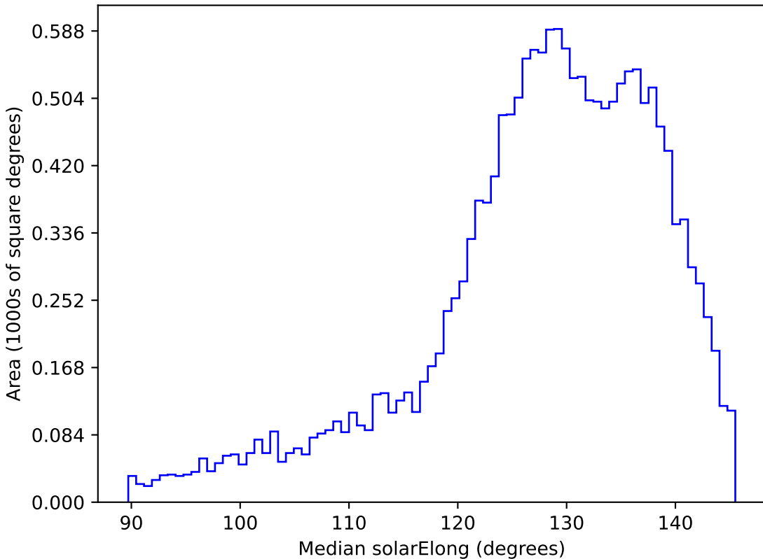
ddf_loaded_fl2_v3.4_10yrs WFD z band: Median solarElong
