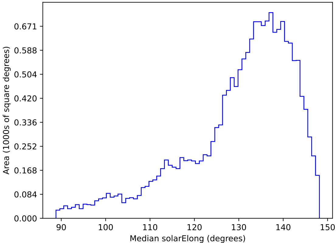
ddf_loaded_fl2_v3.4_10yrs WFD y band: Median solarElong
