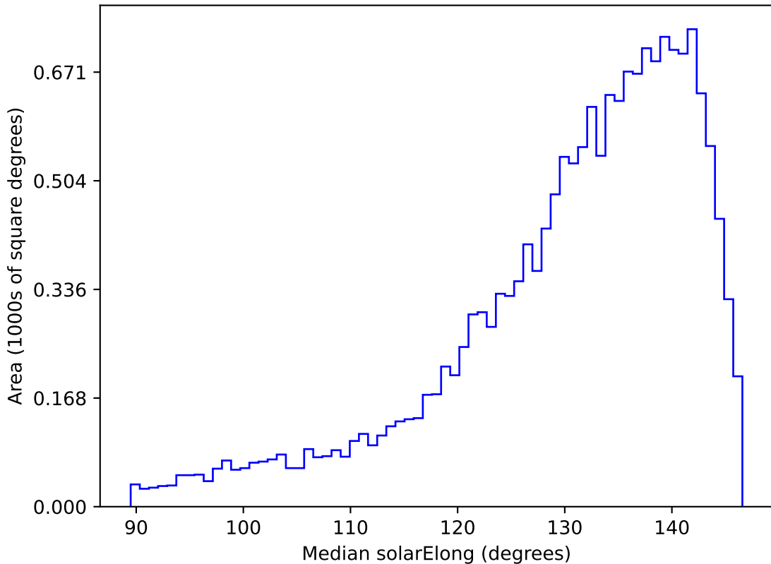
ddf_loaded_fl2_v3.4_10yrs WFD r band: Median solarElong
