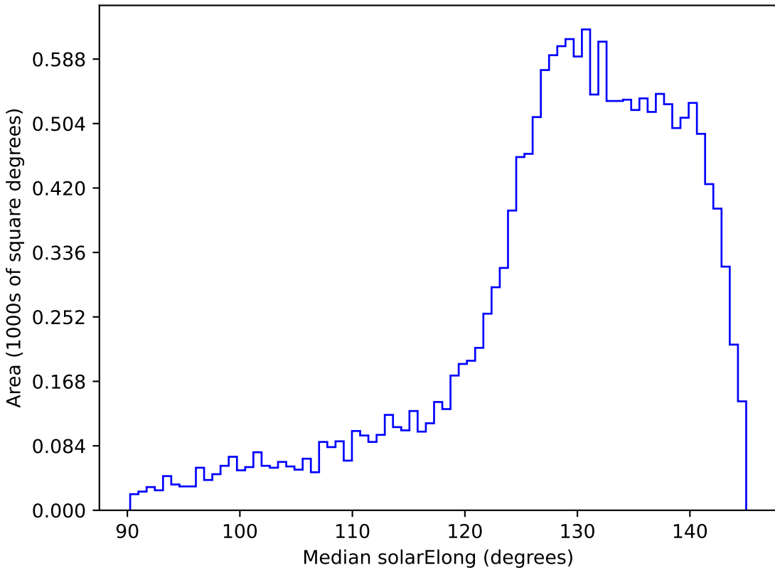
ddf_loaded_fl2_v3.4_10yrs WFD i band: Median solarElong
