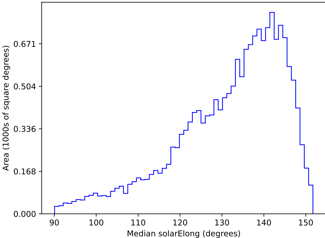
ddf_loaded_fl2_v3.4_10yrs WFD g band: Median solarElong
