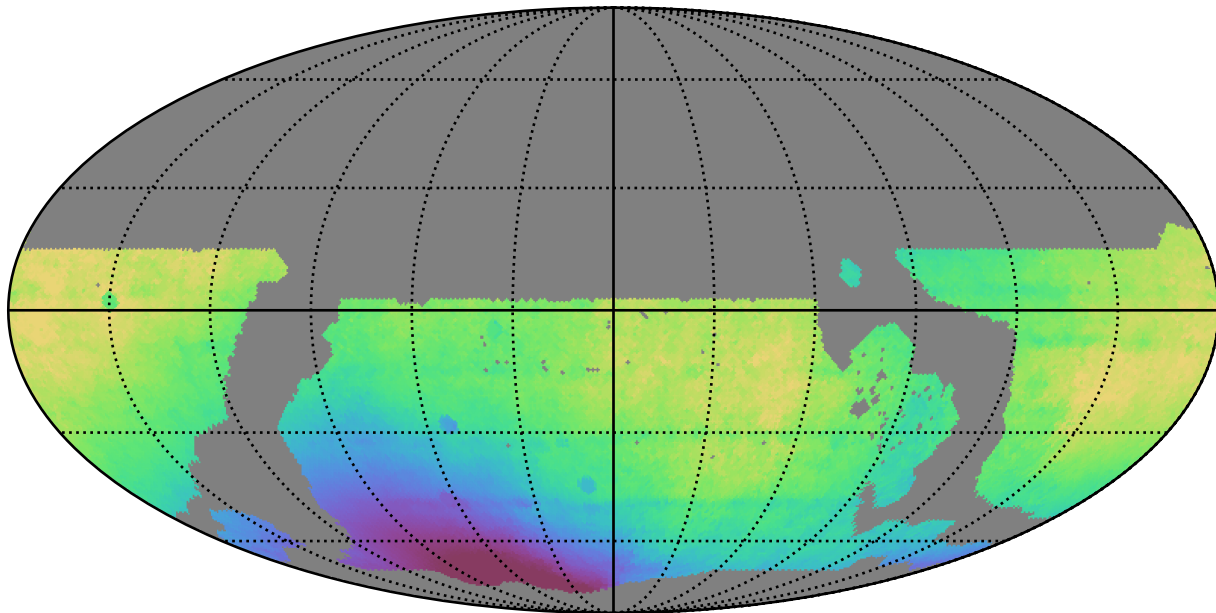
ddf_loaded_fl2_v3.4_10yrs WFD all bands: Median solarElong
