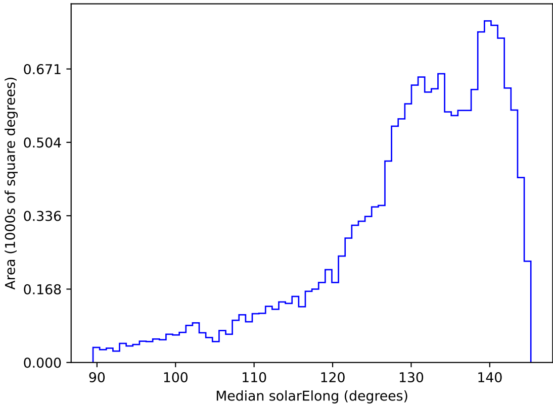
ddf_loaded_fl2_v3.4_10yrs WFD all bands: Median solarElong
