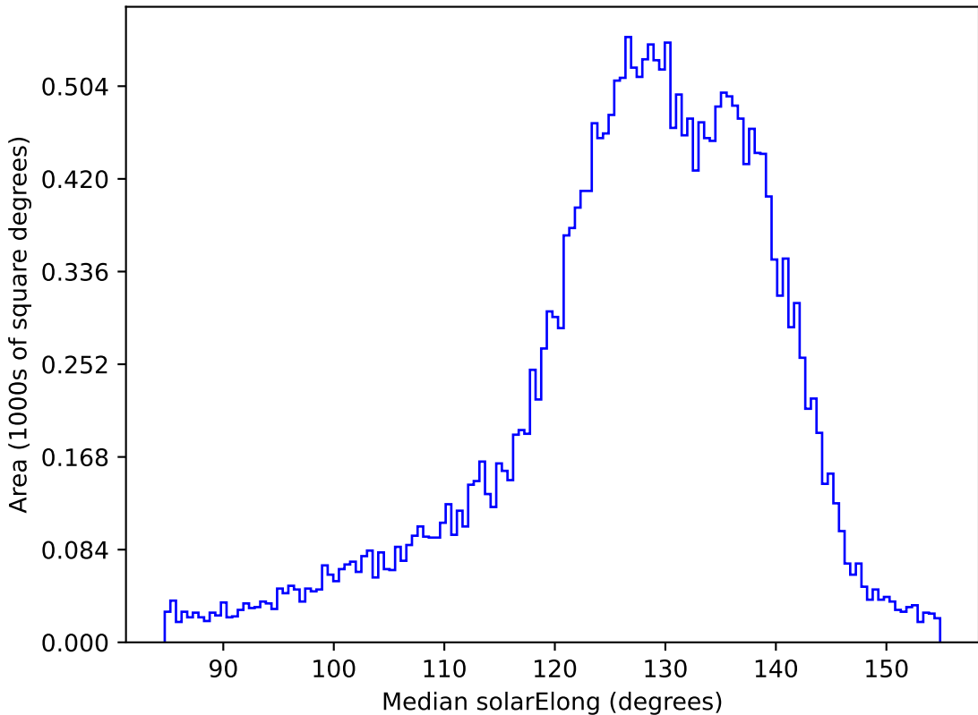
ddf_loaded_fl2_v3.4_10yrs All sky z band: Median solarElong
