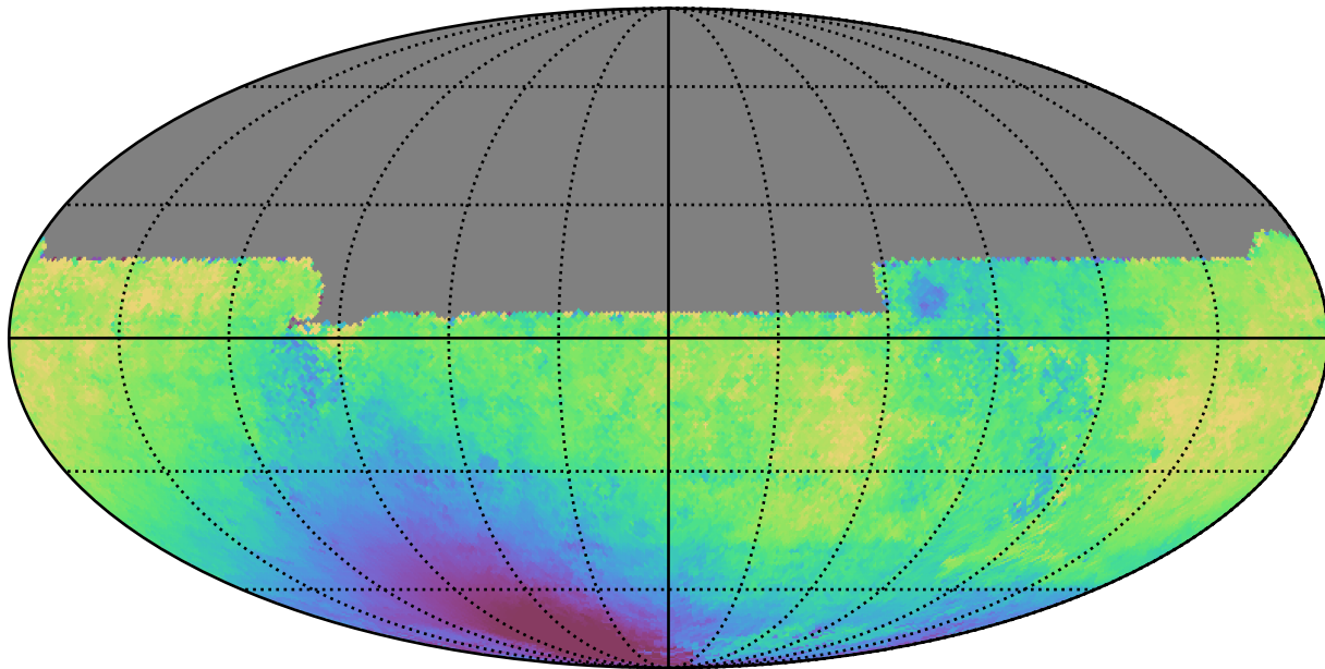
ddf_loaded_fl2_v3.4_10yrs All sky y band: Median solarElong
