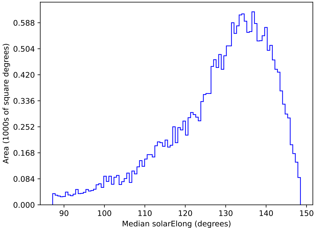
ddf_loaded_fl2_v3.4_10yrs All sky y band: Median solarElong
