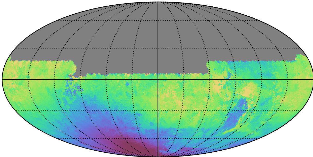
ddf_loaded_fl2_v3.4_10yrs All sky u band: Median solarElong
