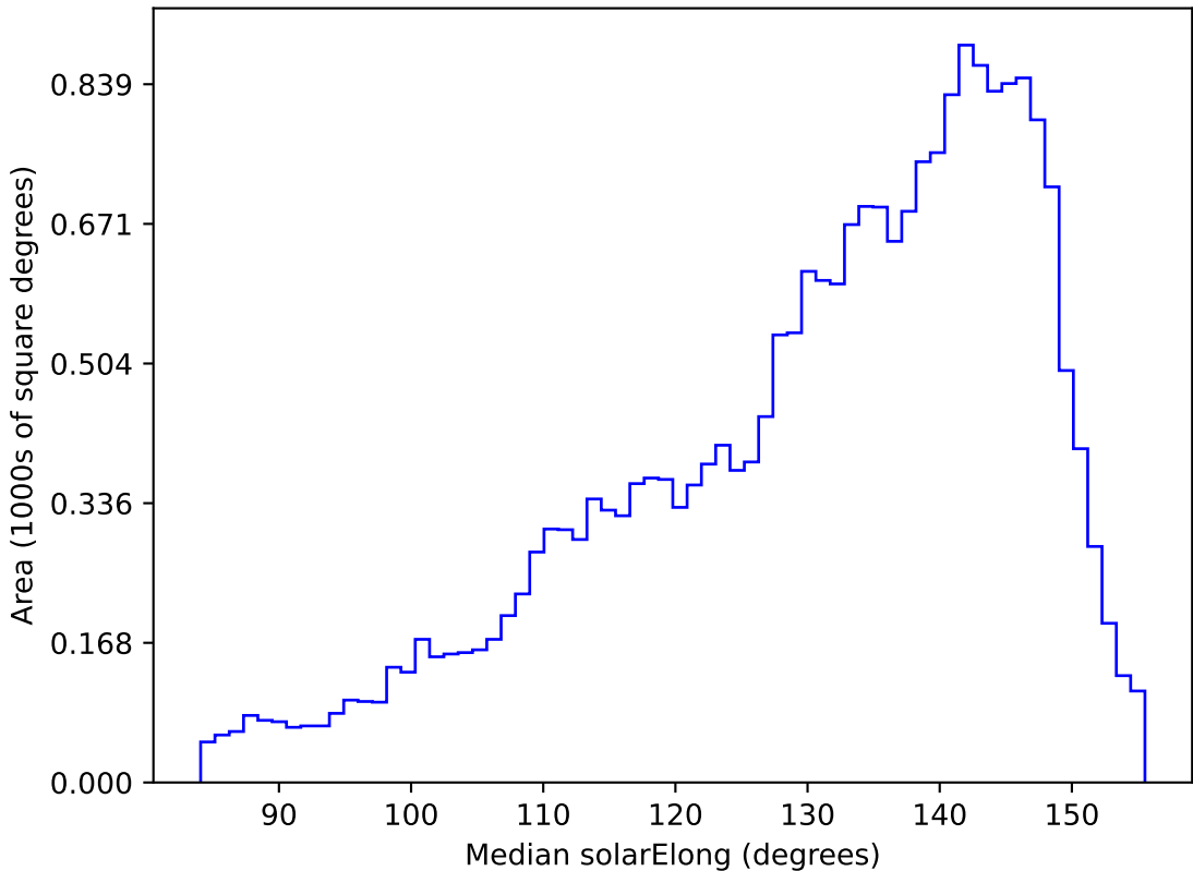
ddf_loaded_fl2_v3.4_10yrs All sky u band: Median solarElong
