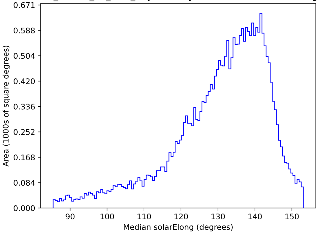
ddf_loaded_fl2_v3.4_10yrs All sky r band: Median solarElong
