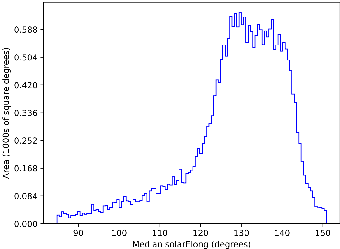
ddf_loaded_fl2_v3.4_10yrs All sky i band: Median solarElong
