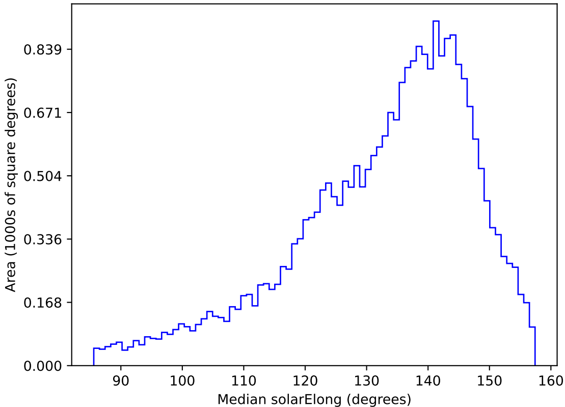
ddf_loaded_fl2_v3.4_10yrs All sky g band: Median solarElong
