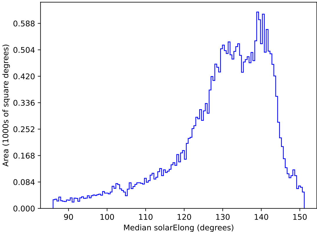
ddf_loaded_fl2_v3.4_10yrs All sky all bands: Median solarElong
