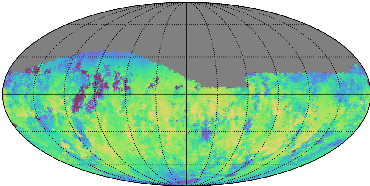
ddf_loaded_fl2_v3.4_10yrs Yr 1 z band: Median skyBrightness
