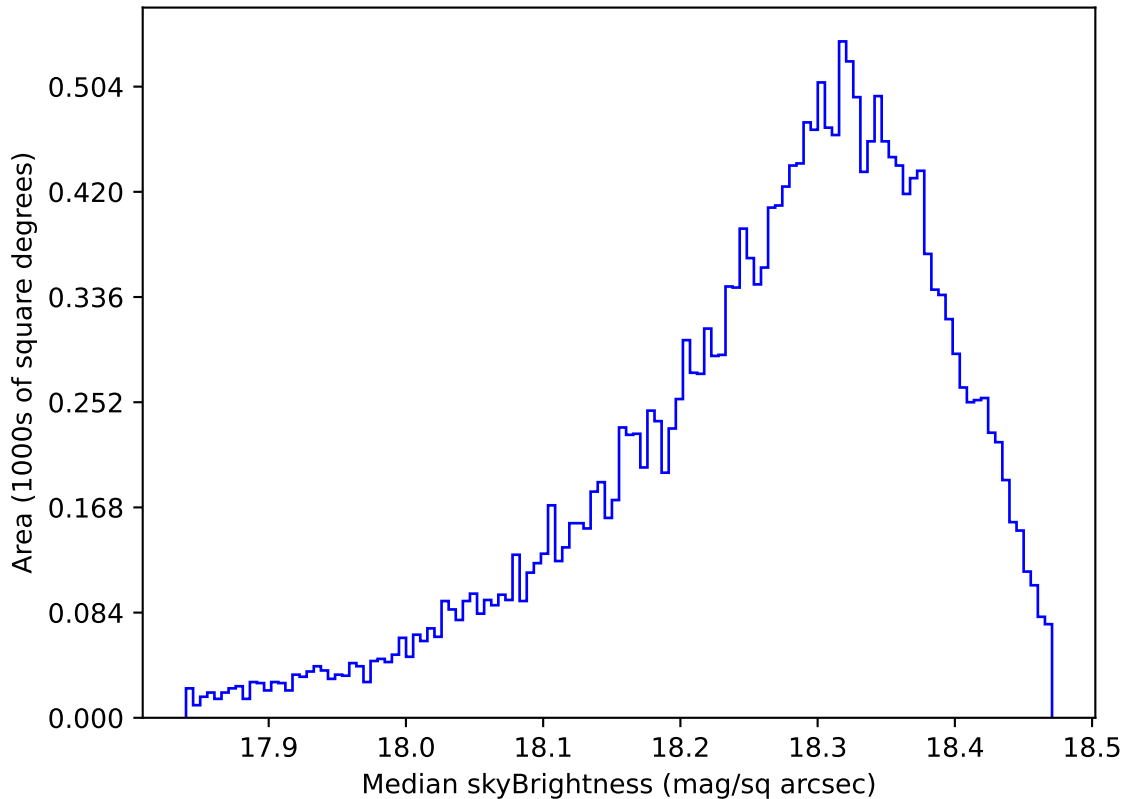
ddf_loaded_fl2_v3.4_10yrs Yr 1 y band: Median skyBrightness
