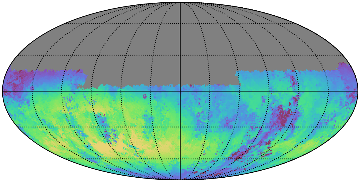
ddf_loaded_fl2_v3.4_10yrs Yr 1 u band: Median skyBrightness
