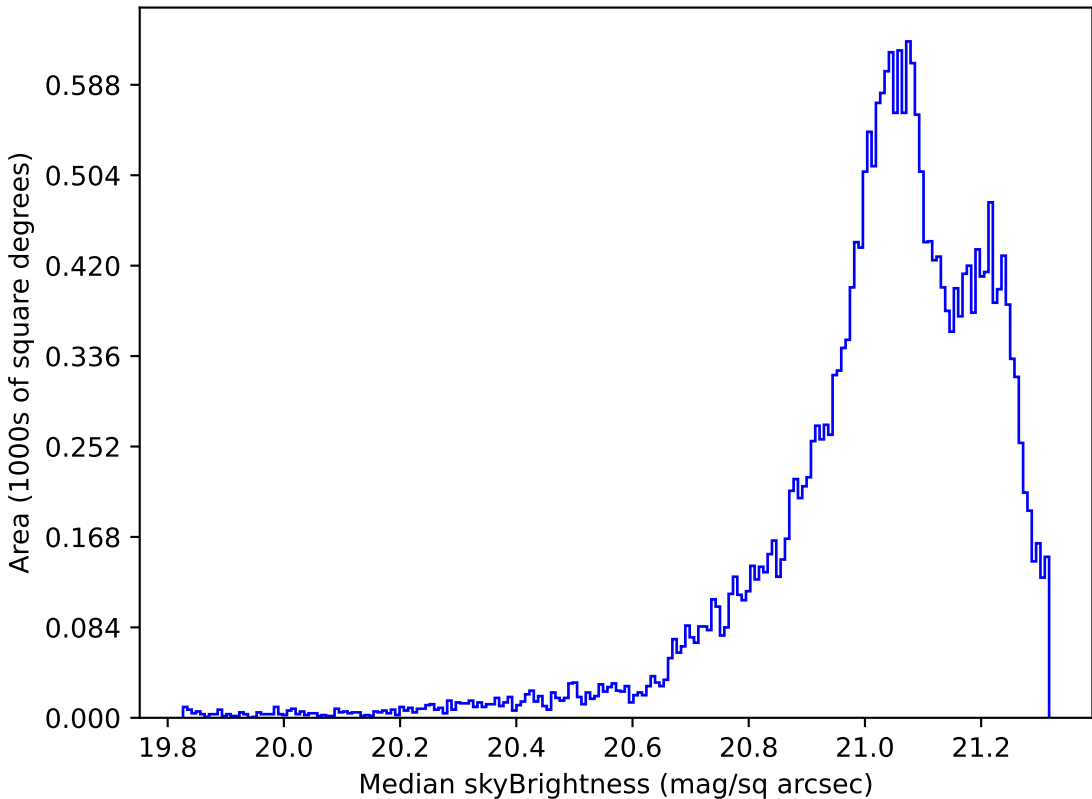
ddf_loaded_fl2_v3.4_10yrs Yr 1 r band: Median skyBrightness
